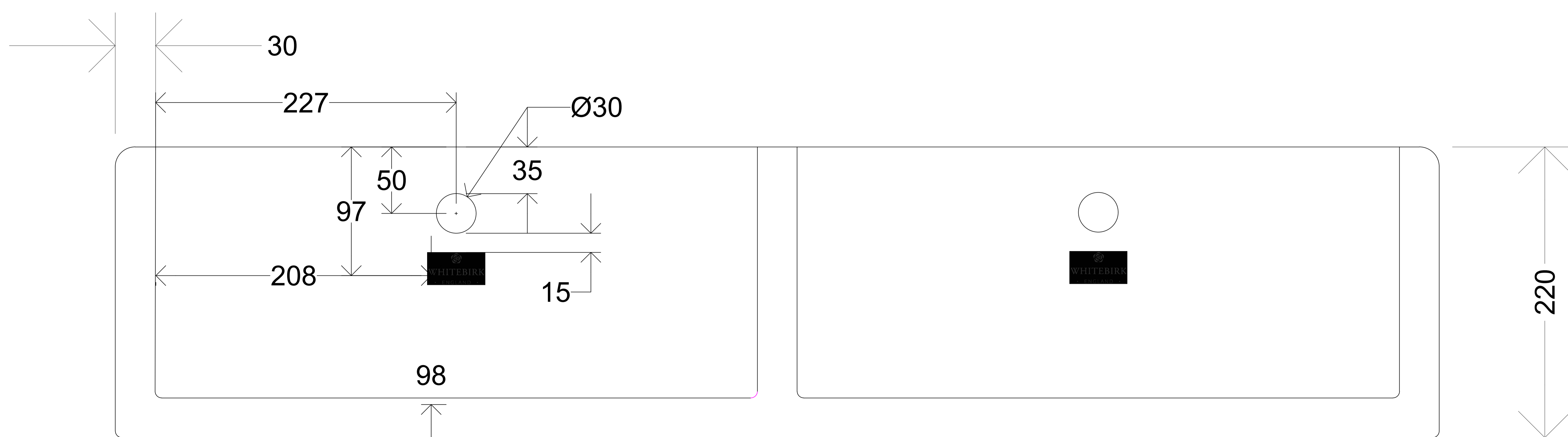
FRONT VIEW
